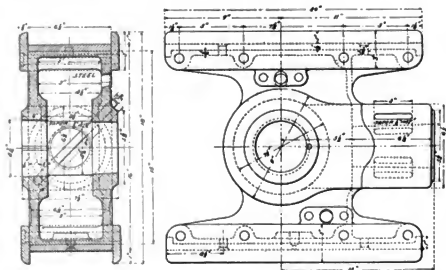
Figs. 1108-1109. Alligator Crosshead.
